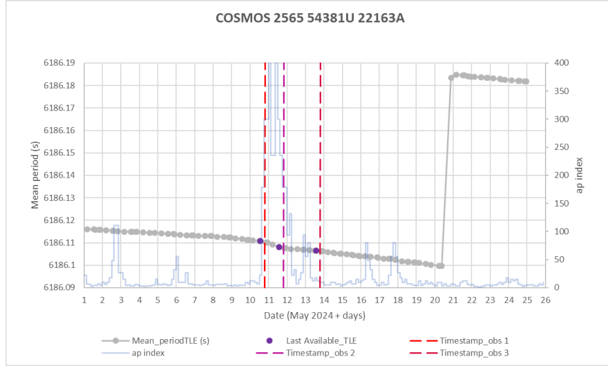
Fig. 5 – Example of an NSM satellite orbital behavior during May 10 - May 20, 2024, followed by an active maneuver on May 20, 2024.
