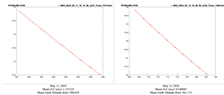
Fig. 15 – Comparison between observed (o) and computed (+) positions for Starklink-5793, on May 11 and on May 13.
