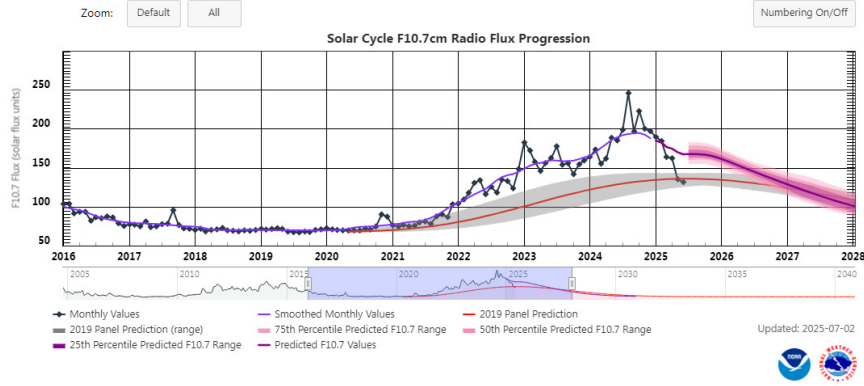
Fig. 1 – The Radio Flux Progression F10.7cm for the current solar cycle, with a May 2024 monthly value of 188.37 Solar Flux Unit, positioned on the increasing branch of the maximum (from NOAA, 2025).
