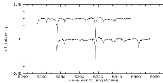
Fig. 3 – Fe II lines in the spectrum of HD 179343.
